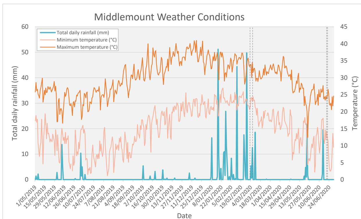
Figure 8: Precipitation/temperature recorded at Middelmount over the previous year (survey period marked with dotted line)
